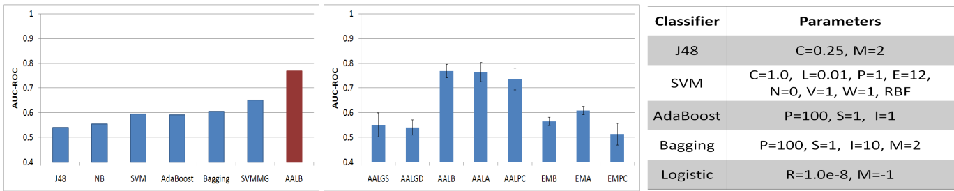
Fig. 3. Classification performances in terms of “Area under the ROC curve” of the different algorithms: (a) propositional classifiers (blue) compared against the relational AALB (red), and (b) relational classifiers. (c) Parameter settings for propositional classifiers
