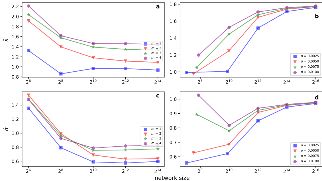
Fig. 4 Dependence in the selection of the embedding dimension from network size and density. a \hat{s} as a function of the network size N in the BA model. We control the network size and change network density of BA model by choosing different number of edges to attach from a new node to the existing nodes. c \hat{\alpha} as a function of the network size for the same networks as in (a) . b, d Same as in panels a and c , respectively, but for the ER model. Here, we control the density of the graphs by tuning the link probability p between different nodes.
